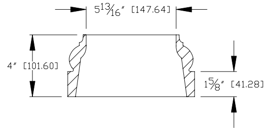
SECTION A-A SCALE 1: 6
